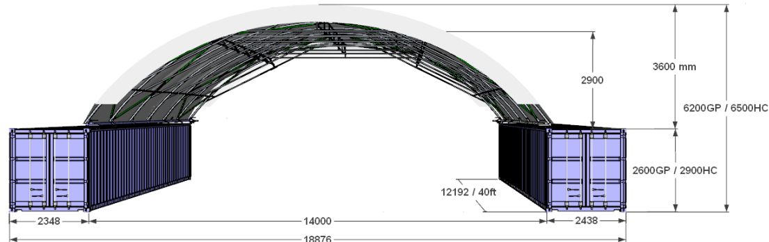
14.0mtr x 40ft - Dome Roof Structure
