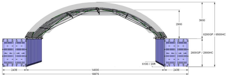
14.0mtr x 20ft - Dome Roof Structure
