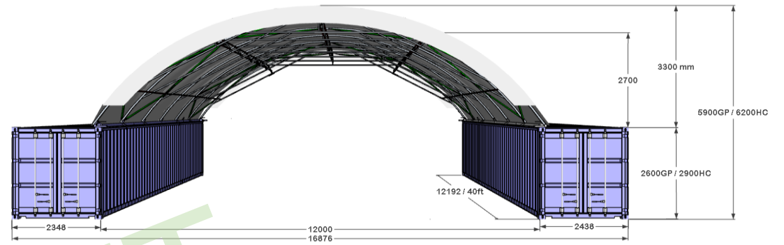
12.0mtr x 40ft - Dome Roof Structure
