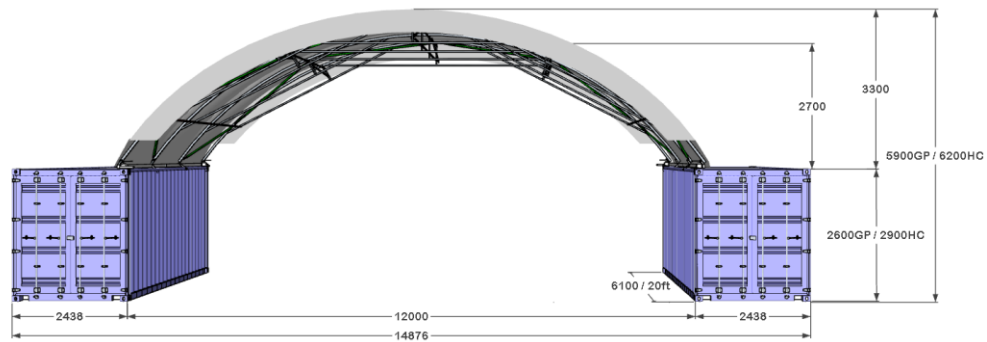
12.0mtr x 20ft - Dome Roof Structure
